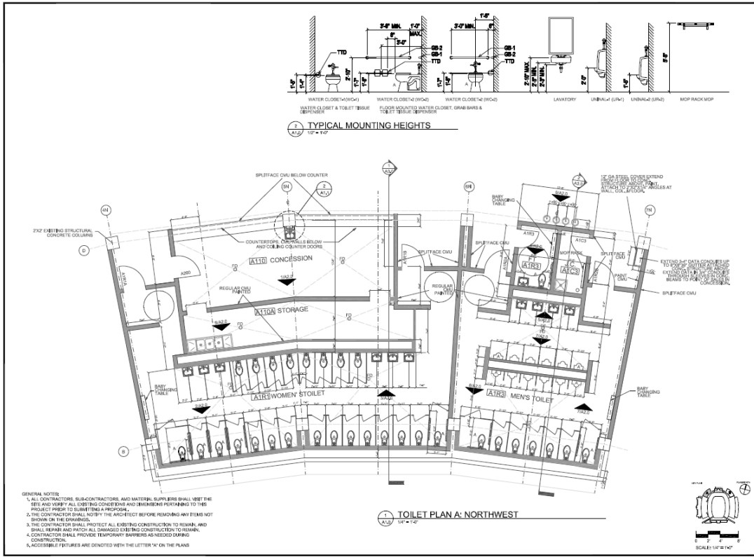
Concessions and Toilet Room Floor Plan
