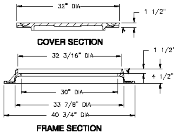
Attachment 1 – Sanitary Sewer Manhole Cover
